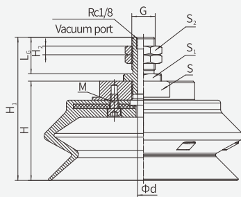
Vertical – Male thread connection
