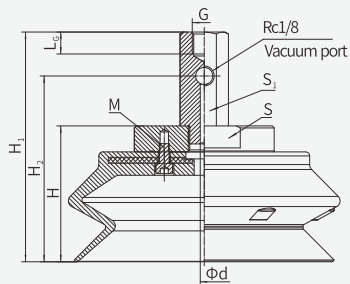
Lateral – Female thread connection
